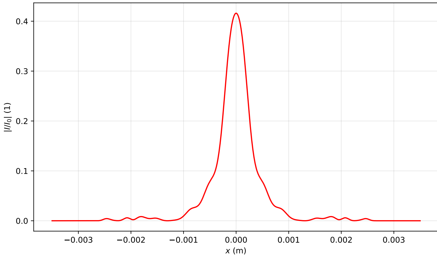
Intensity profile I(x, y = 0, z = 2.388)/I_0 , P_{in}=4.0P_{cr} , artificial time
